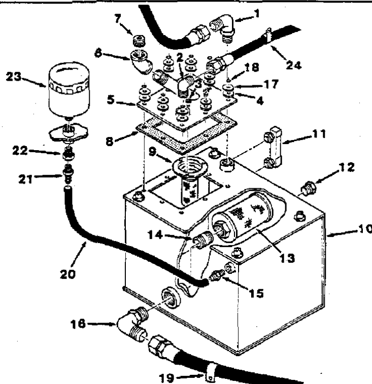
FIG. 18 - HYDRAULIC FLUID RESERVOIR GROUP
