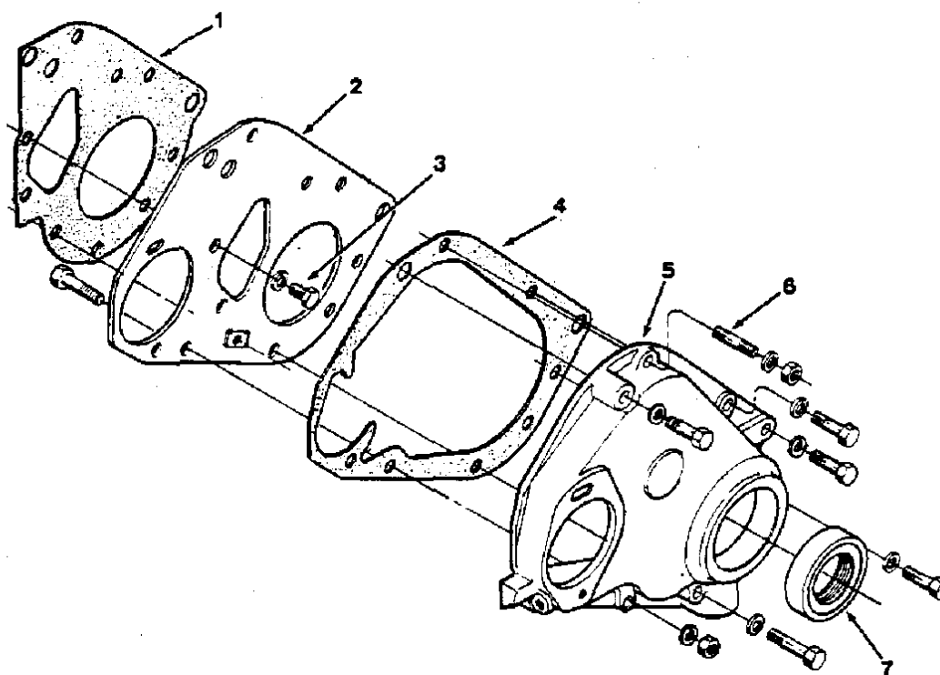
FIG. 4 - FRONT END PLATE AND GEAR COVER GROUP
