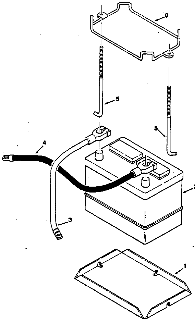
FIG. 6 - BATTERY GROUP
