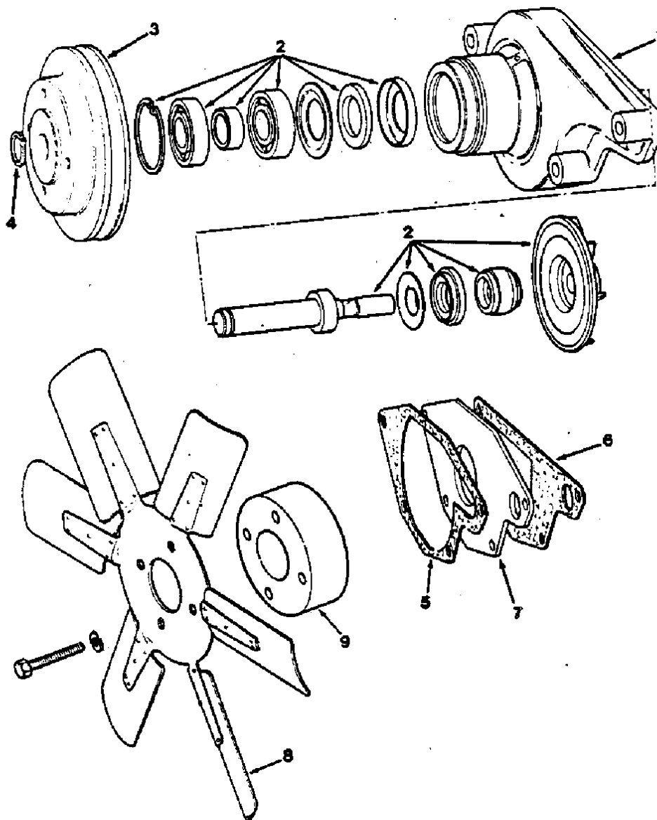
FIG. 8 - WATER PUMP GROUP
