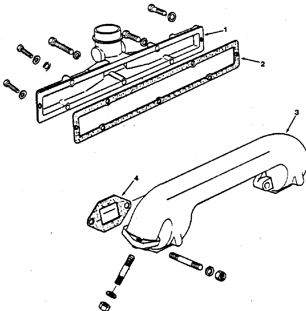
FIG. 4 - MANIFOLD GROUP
