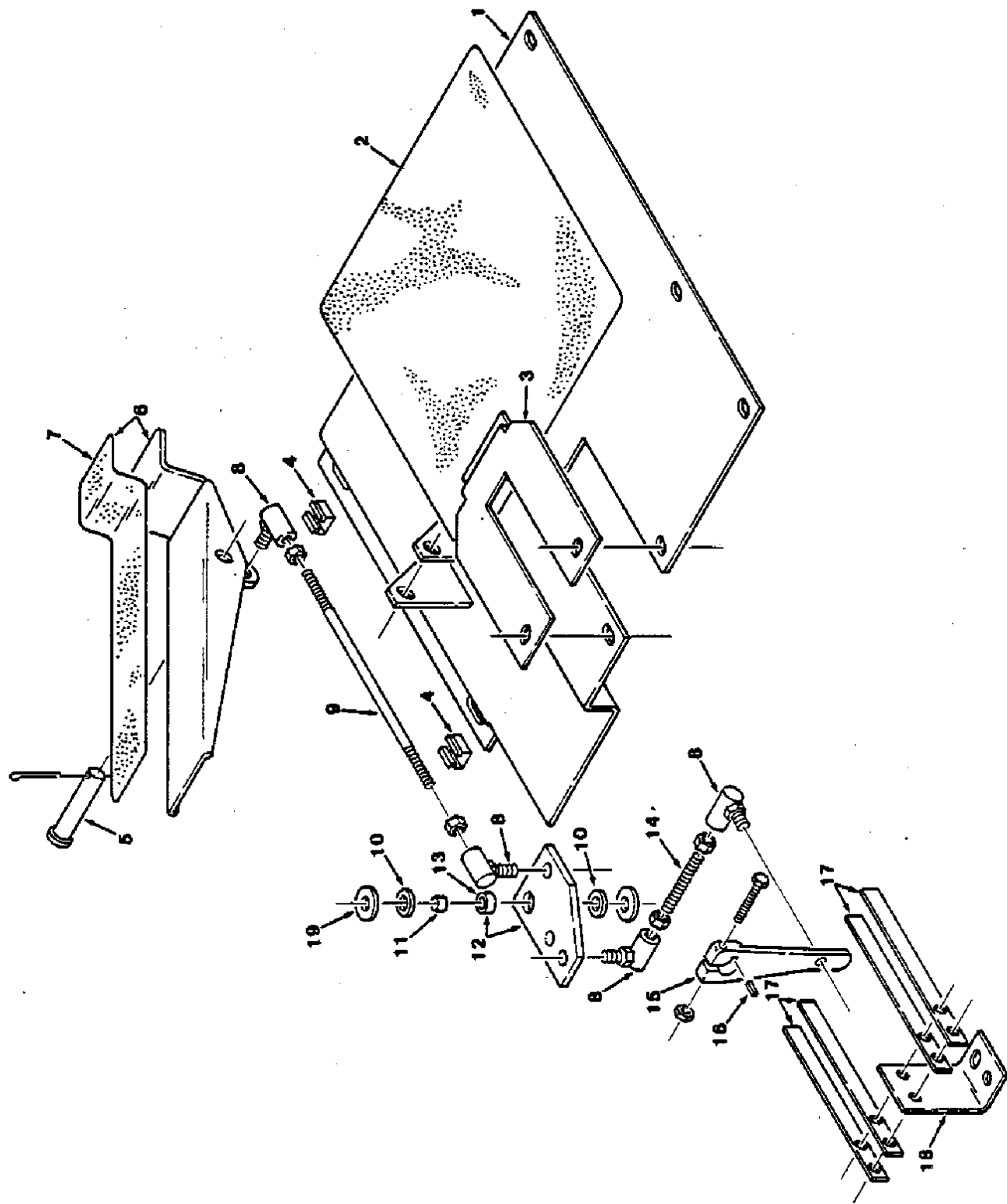
FIG. 7 - DIRECTIONAL CONTROL PEDAL GROUP
