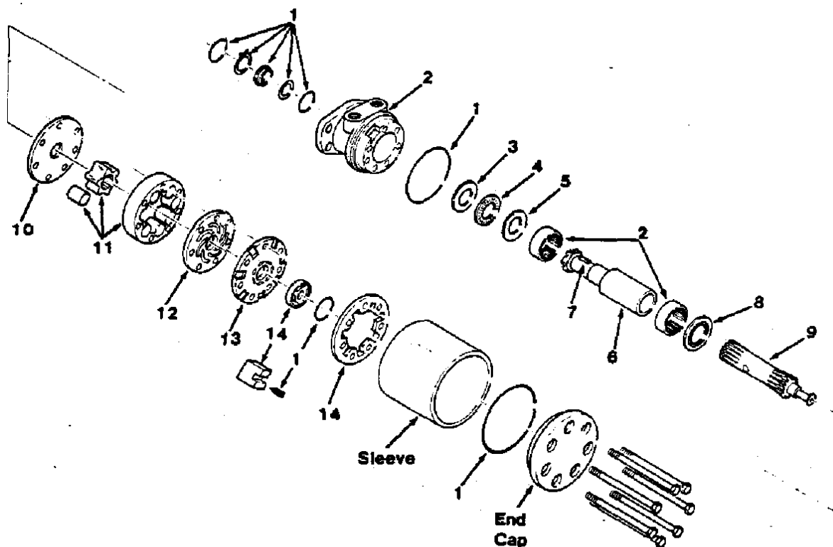
FIG. 4 - HYDRAULIC DRIVE MOTOR BREAKDOWN
