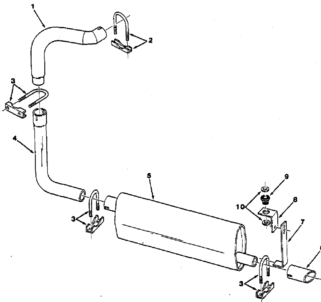
FIG. 10 - EXHAUST SYSTEM GROUP
