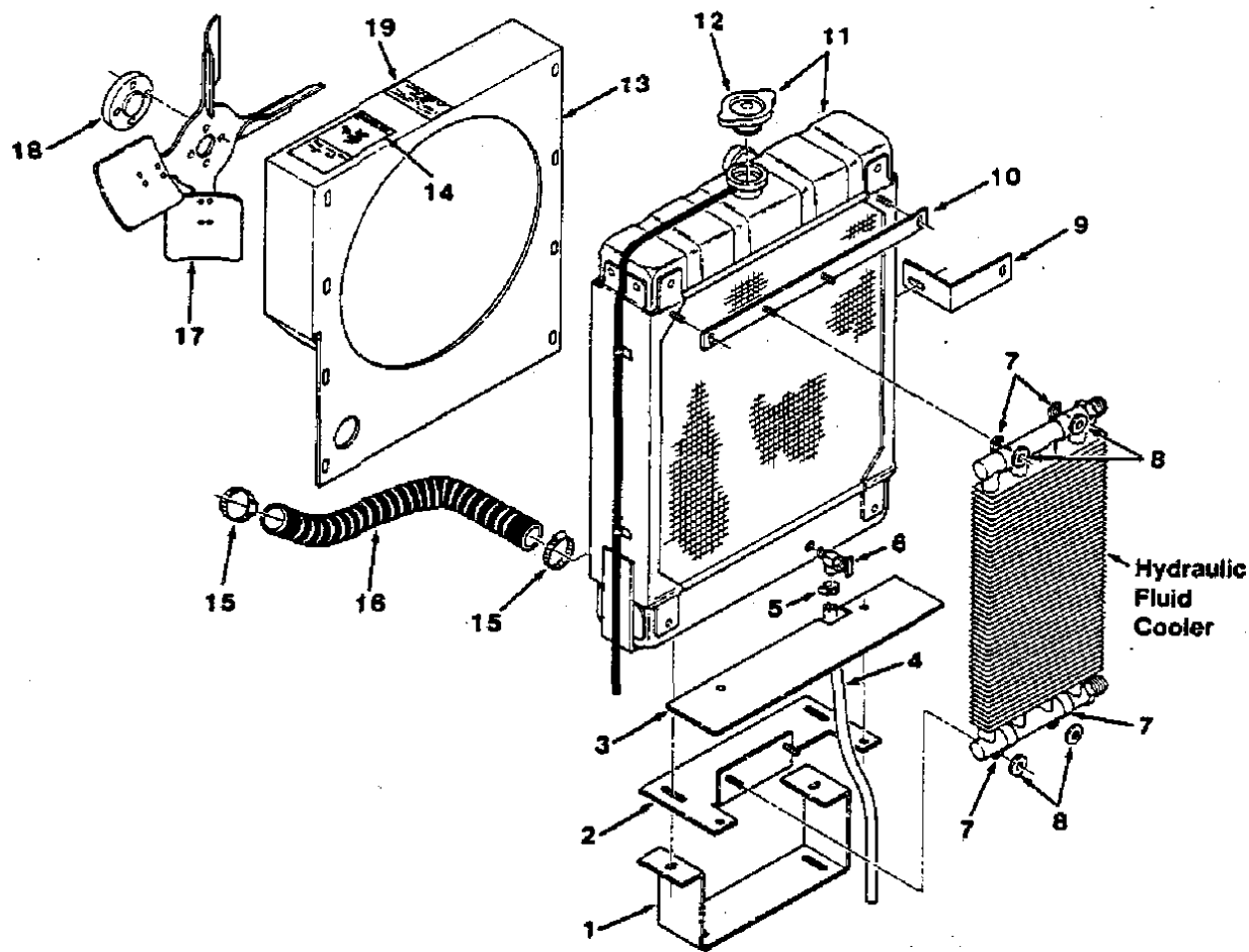
FIG. 11 - RADIATOR GROUP
