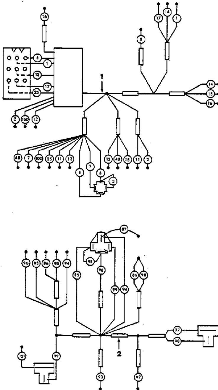
FIG. 34 - WIRE HARNESSES, STANDARD
