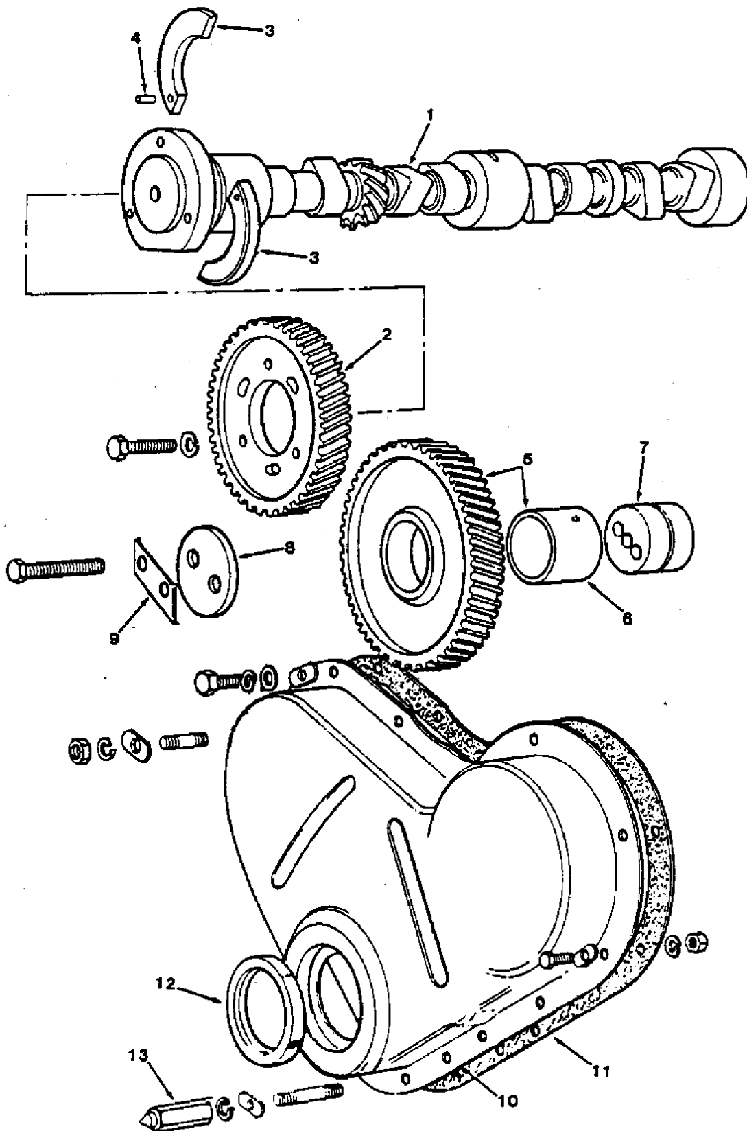
FIG. 8 - TIMING GEAR GROUP
