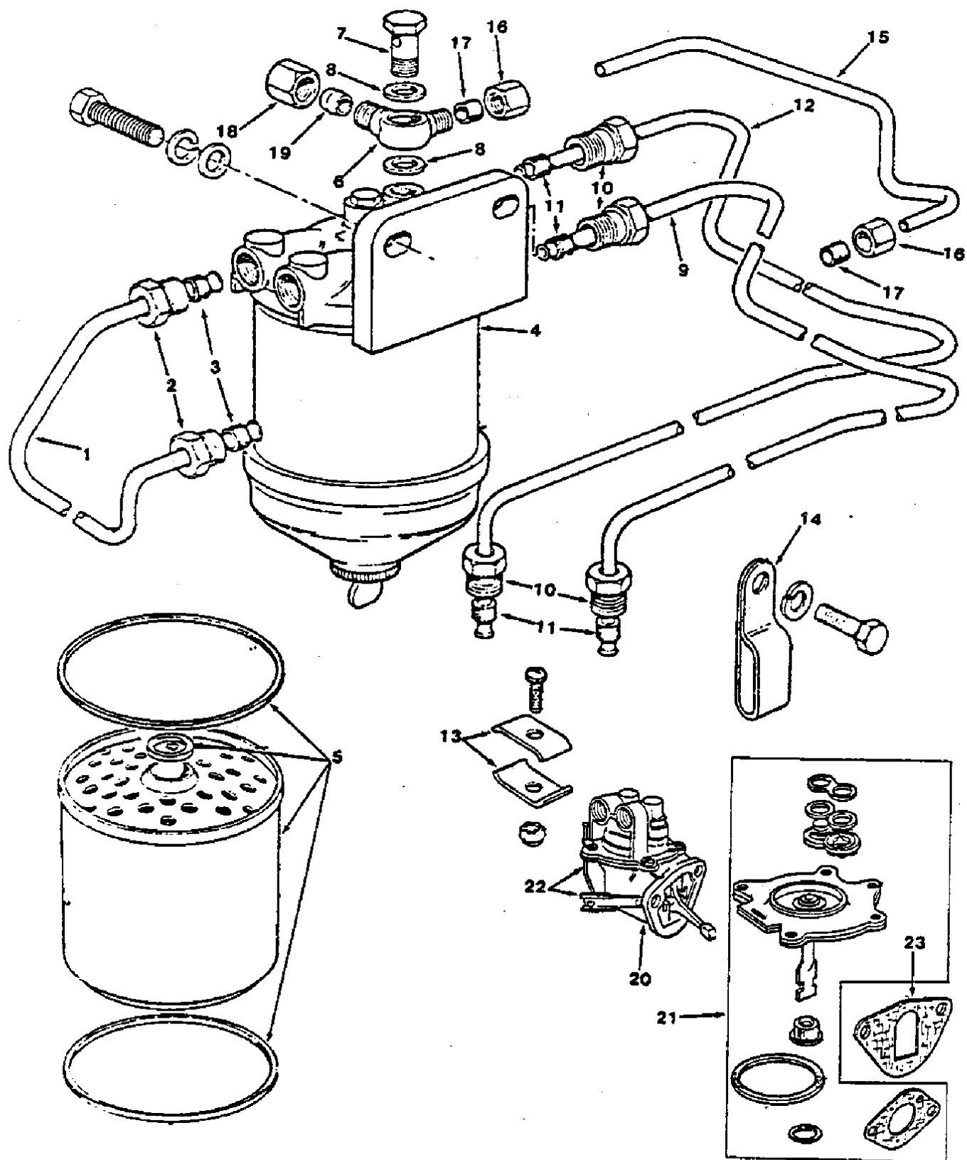
FIG. 10 - FUEL FILTER AND PUMP GROUP
