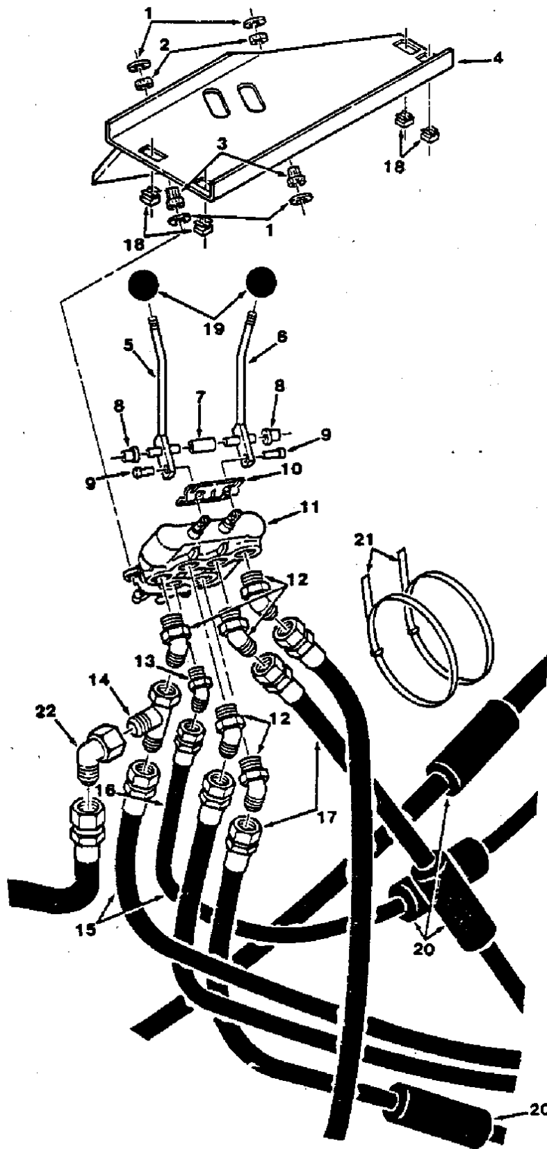
FIG. 20 - CONTROL VALVE PANEL GROUP
