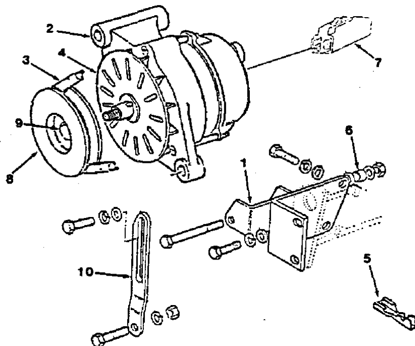
FIG. 9 - ALTERNATOR GROUP
