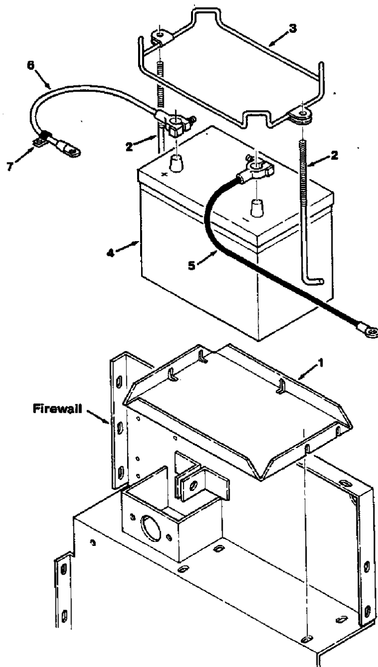
Fig. 8 - Battery Group
