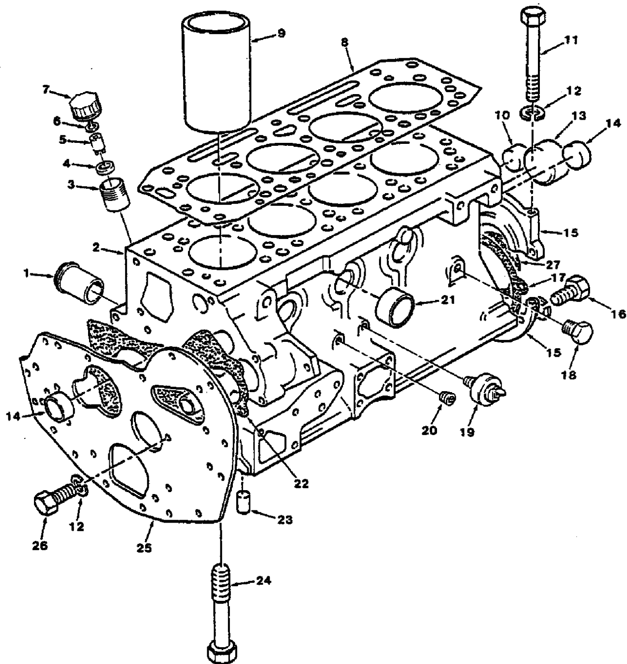
Fig. 1 - Block Group
