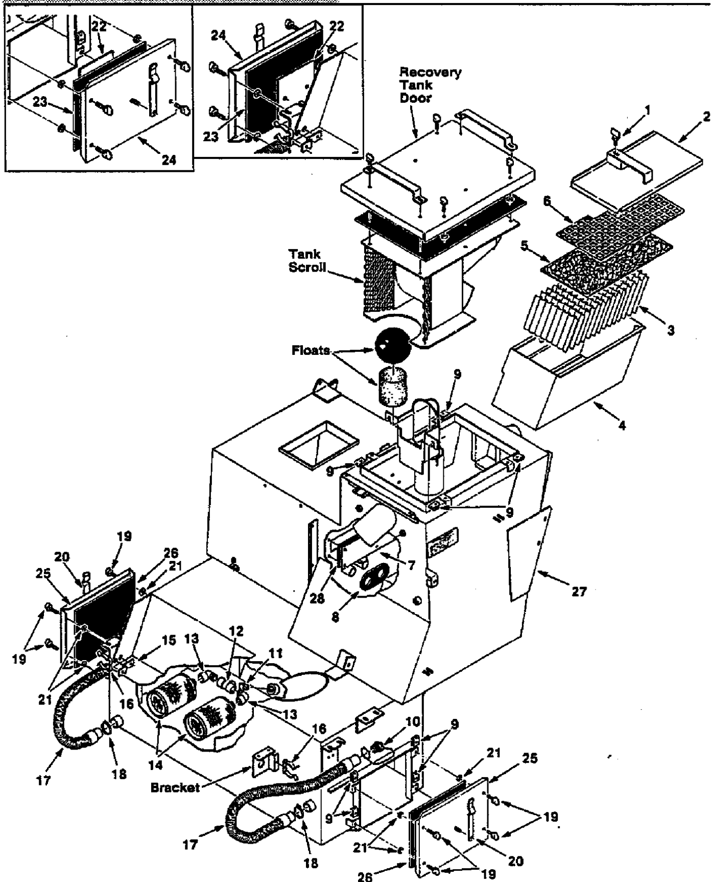
Fig. 2 - Solution and Recovery Tank Group, SRS®
