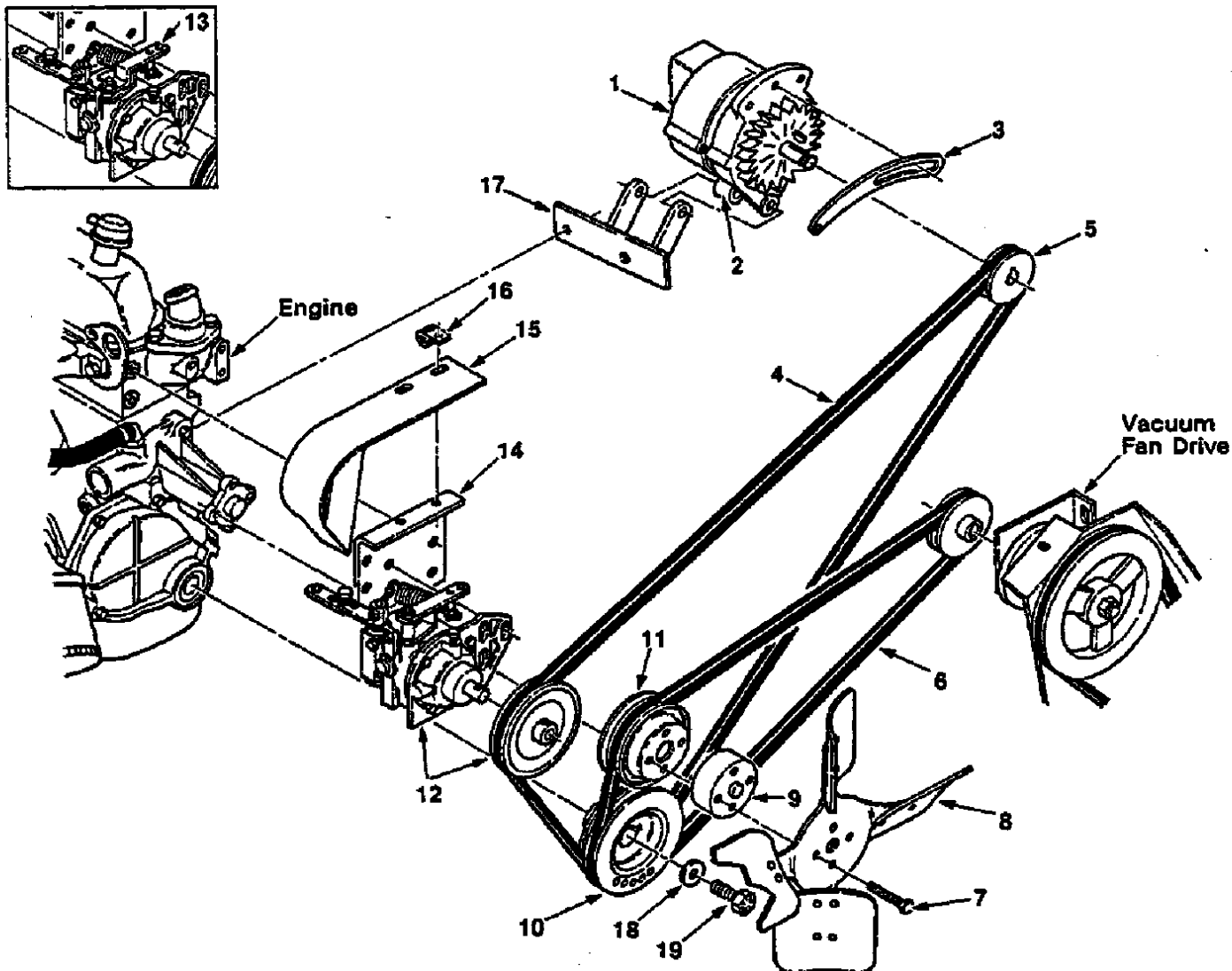
Fig. 15 - Engine Belts Group
