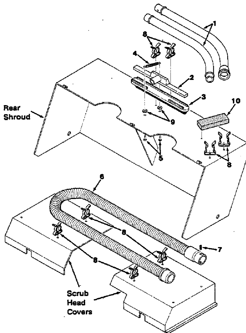
Fig. 15 - Vacuum Wand Kit
