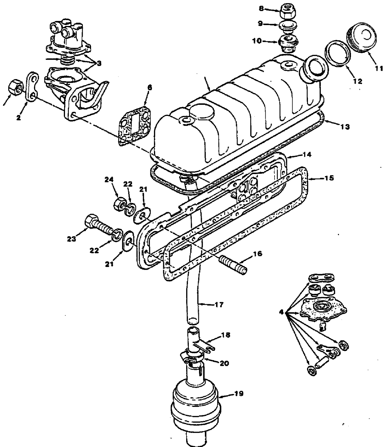
Fig. 4 - Cover Group
