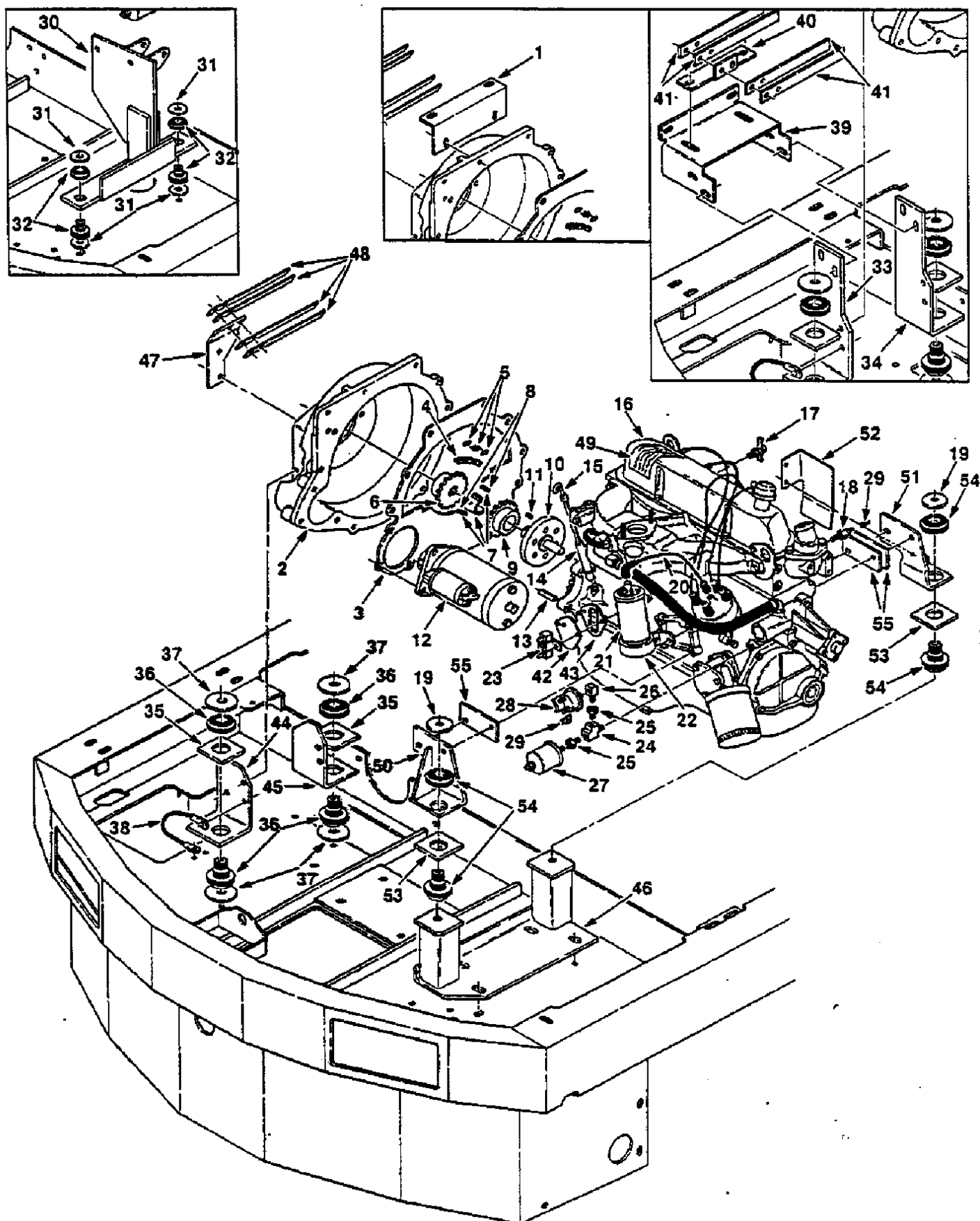
Fig. 14 - Engine Group
