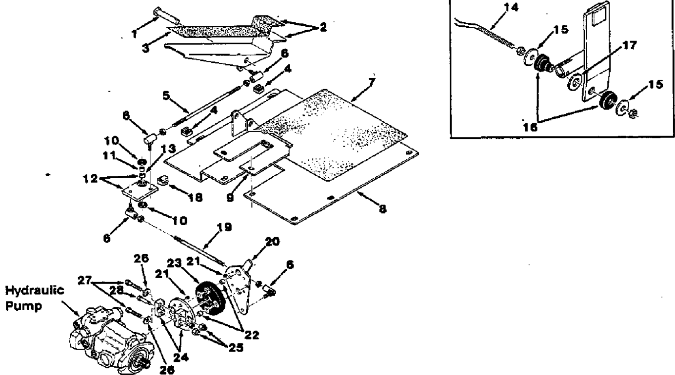
Fig. 7 - Directional Control Group
