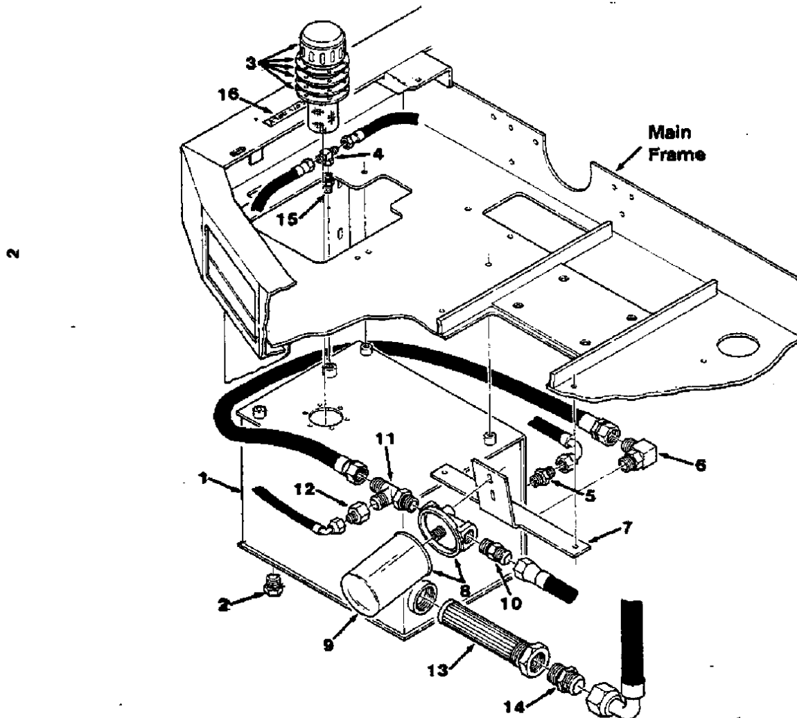
Fig. 8 - Hydraulic Reservoir Group, Diesel
