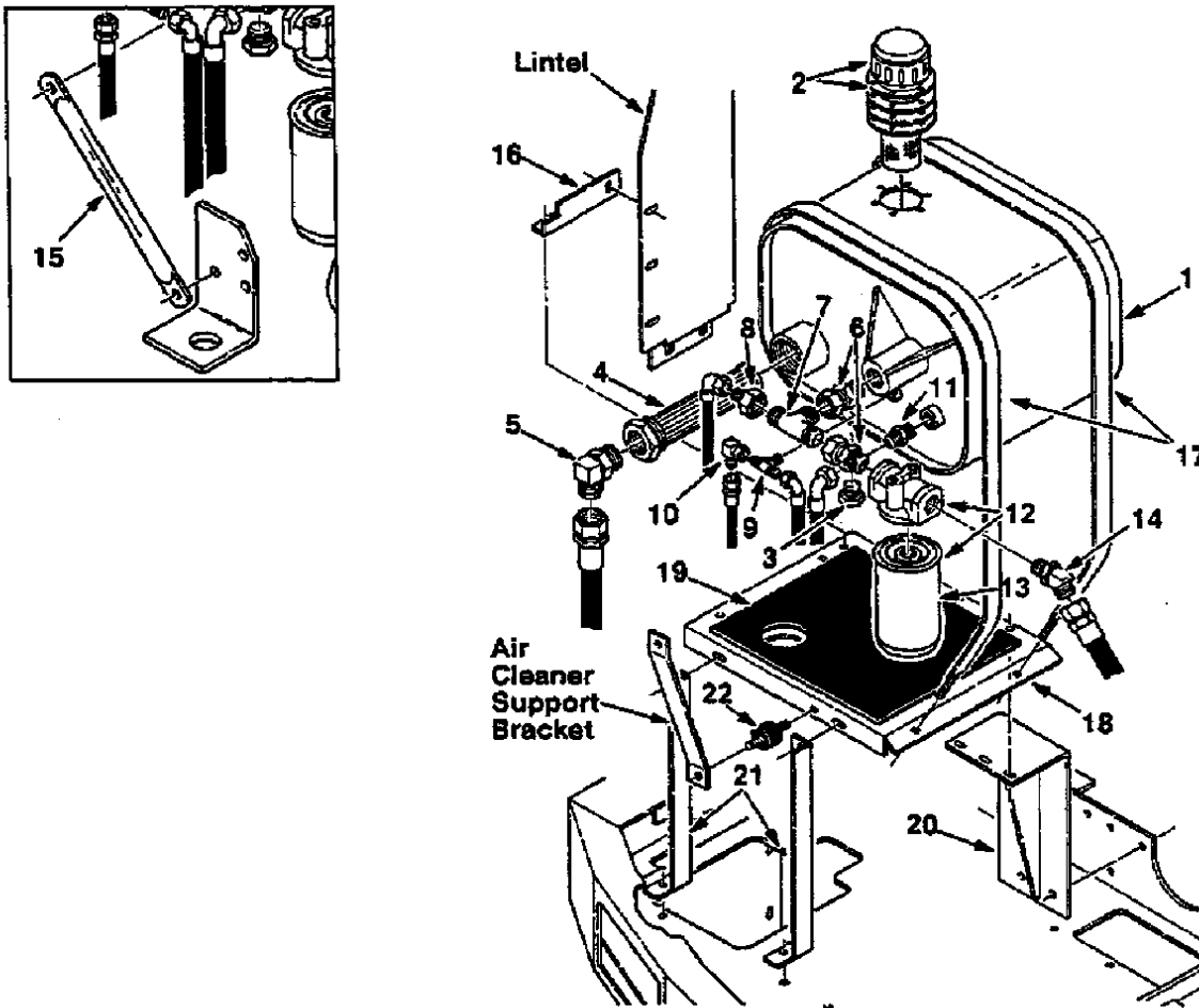
Fig. 20 - Hydraulic Reservoir Group
