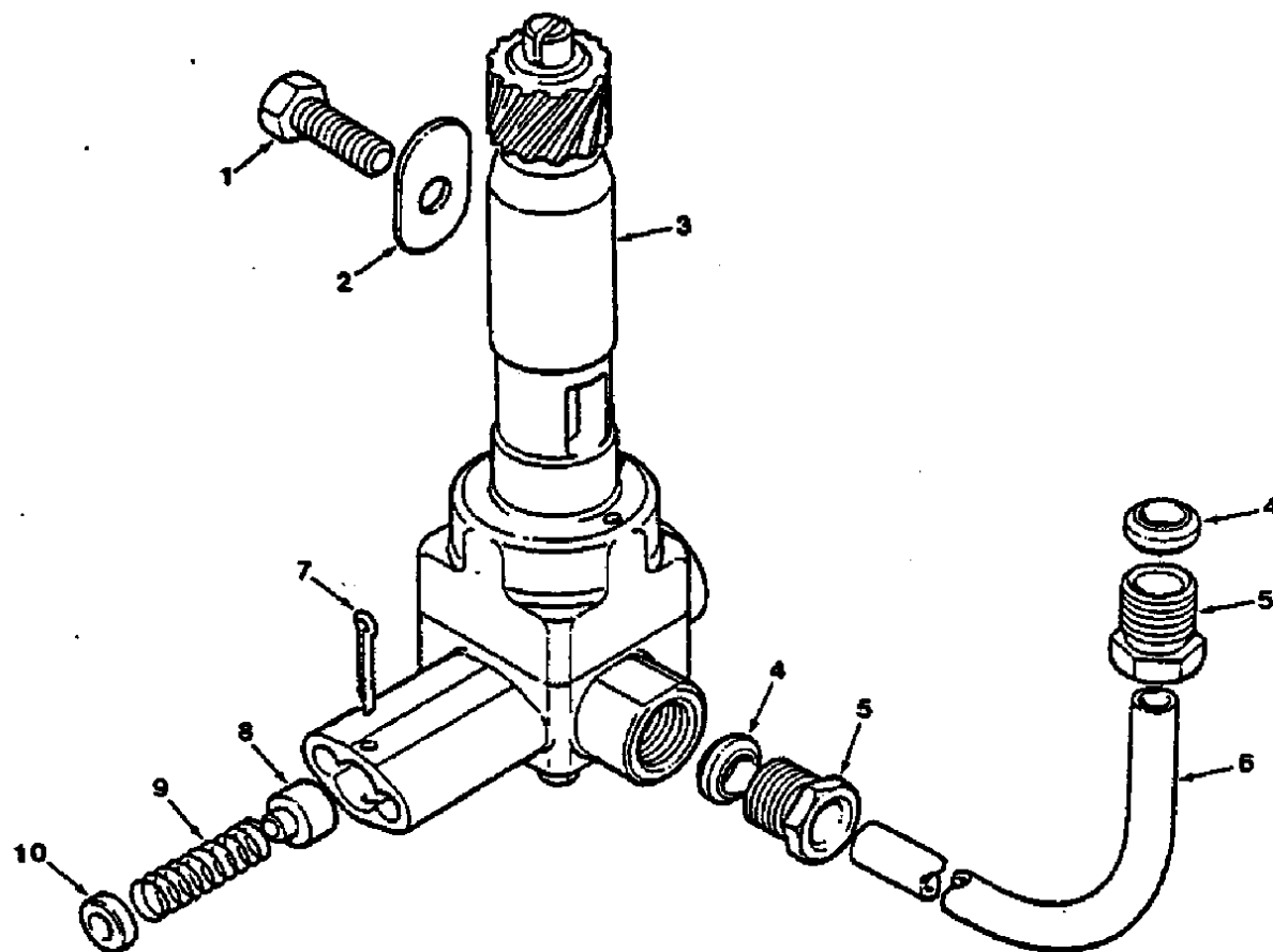
Fig. 10 - Oil Pump Group
