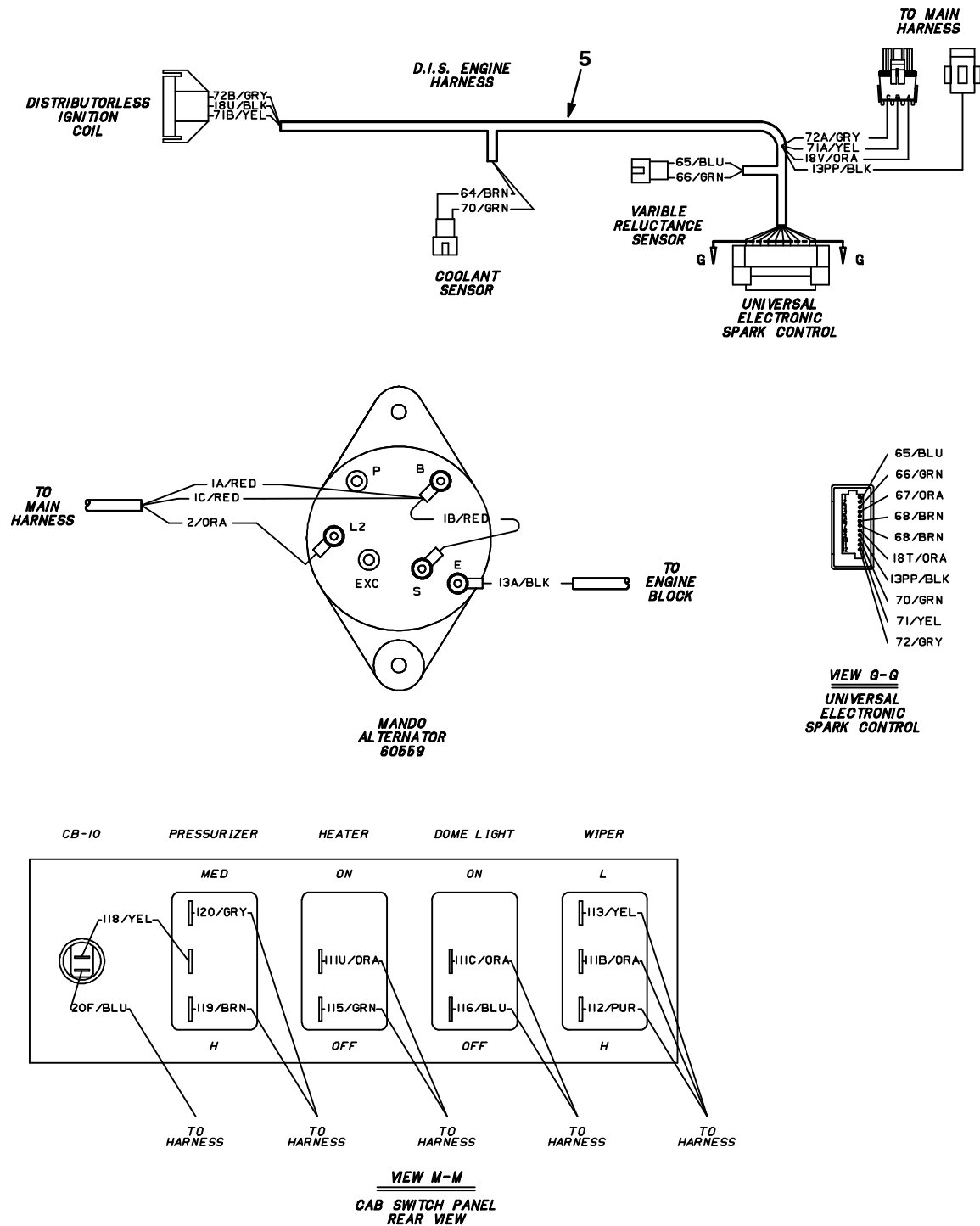
Fig. 59 - Wire Harnesses Group
