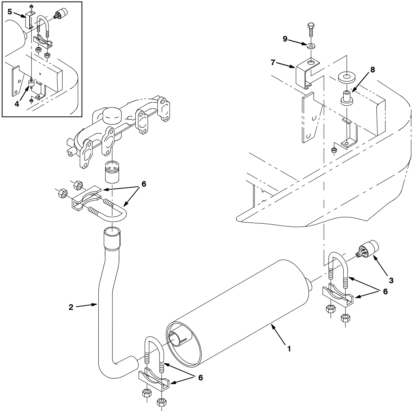
Fig. 22 - Muffler Group
