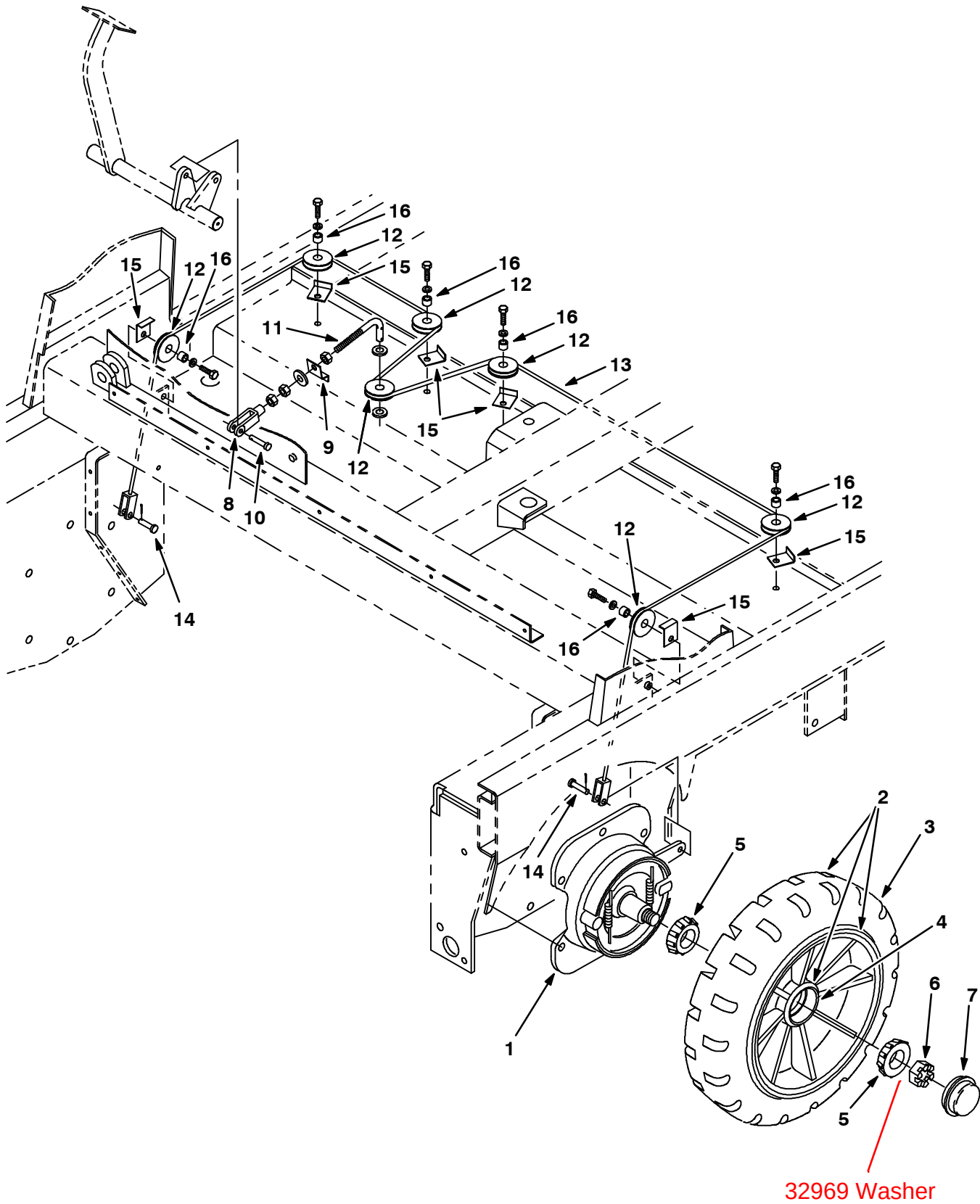
Fig. 34 - Front Wheel and Brakes Group
