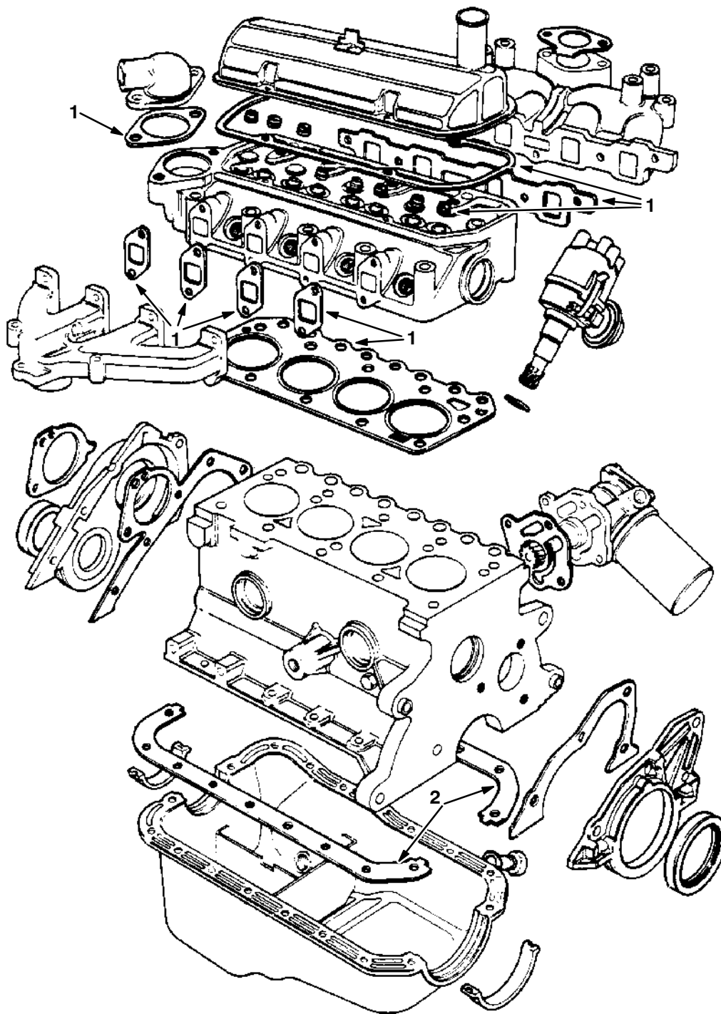
Fig. 10 - Gaskets Group
