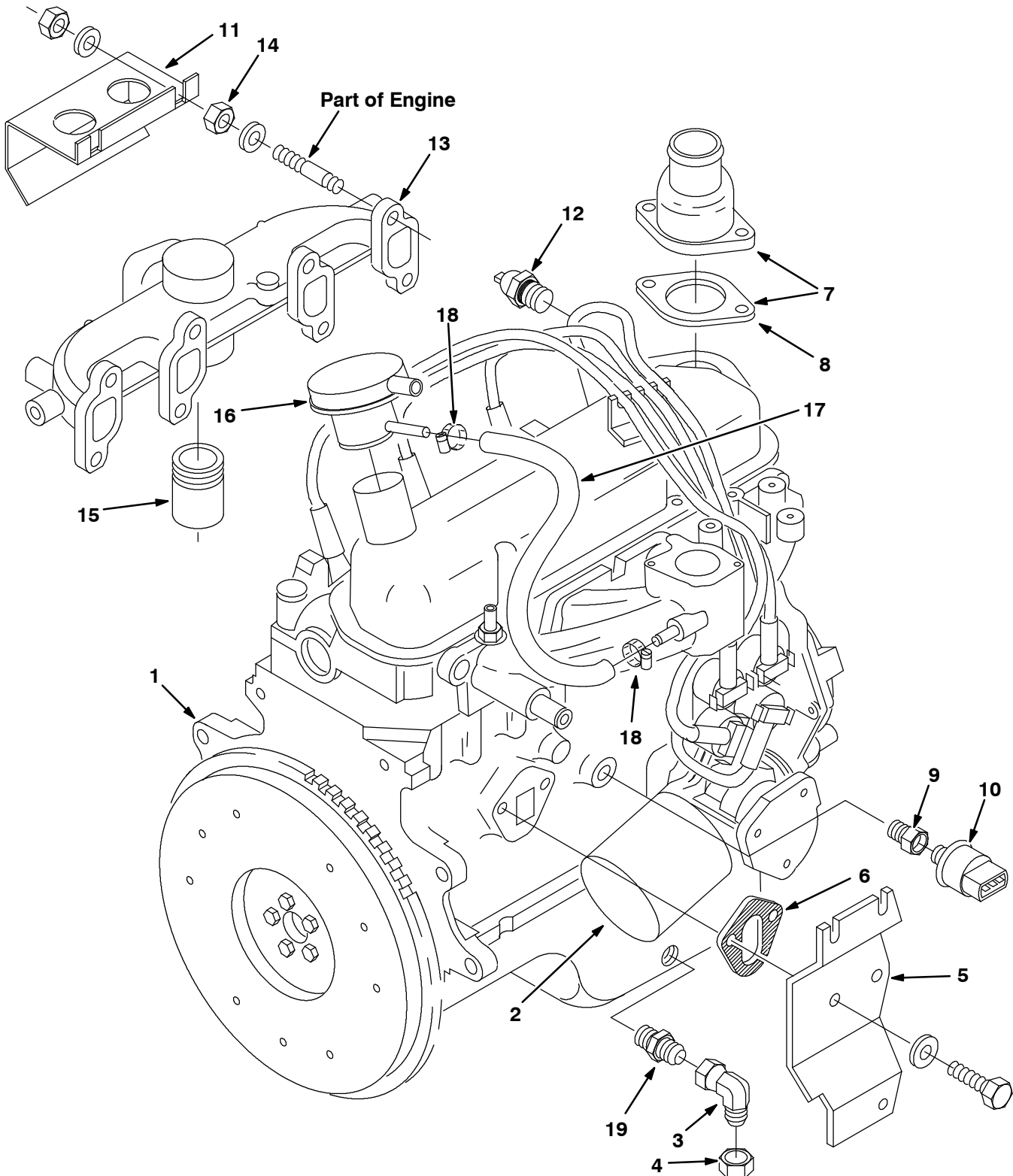
Fig. 15 - Engine Group
