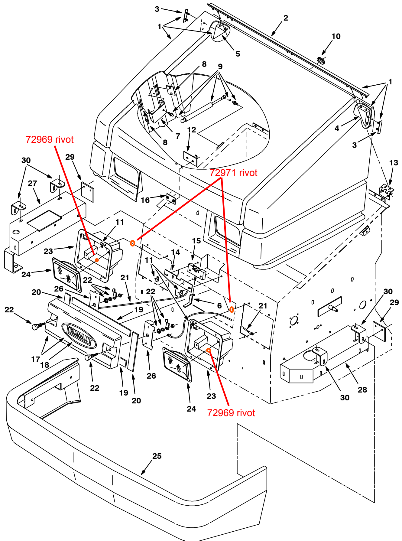
Fig. 40 - Hopper Hood and Bumper Group
