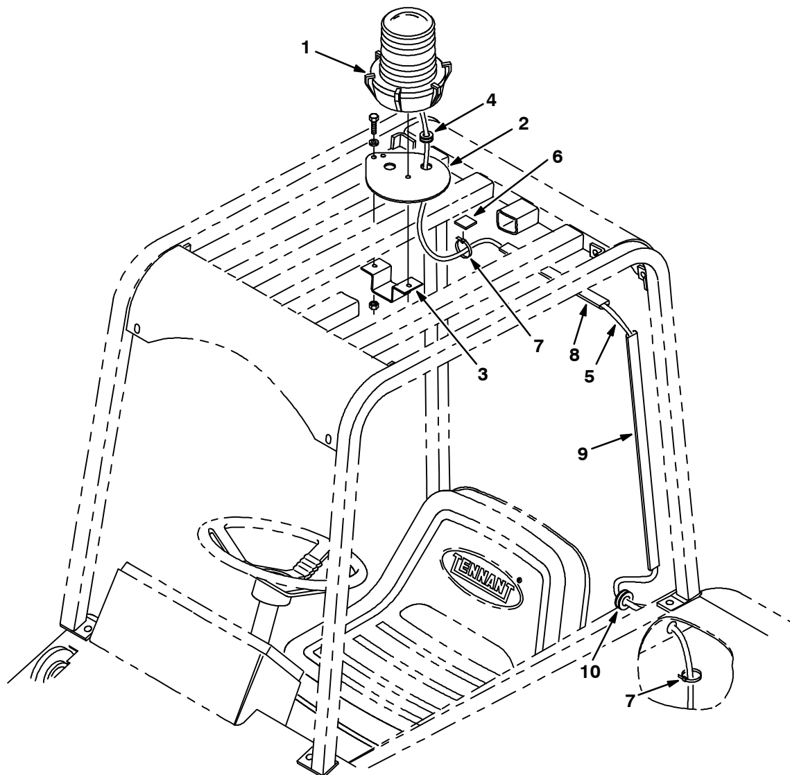
Fig. 2 - Flashing Light Kit, Overhead Guard
