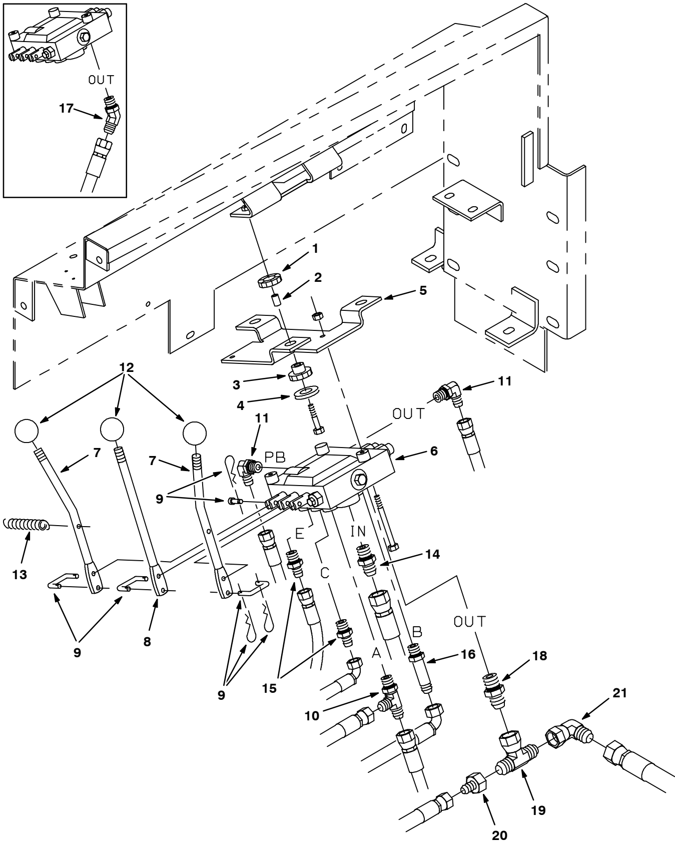
Fig. 54 - Hydraulic Valve Group
