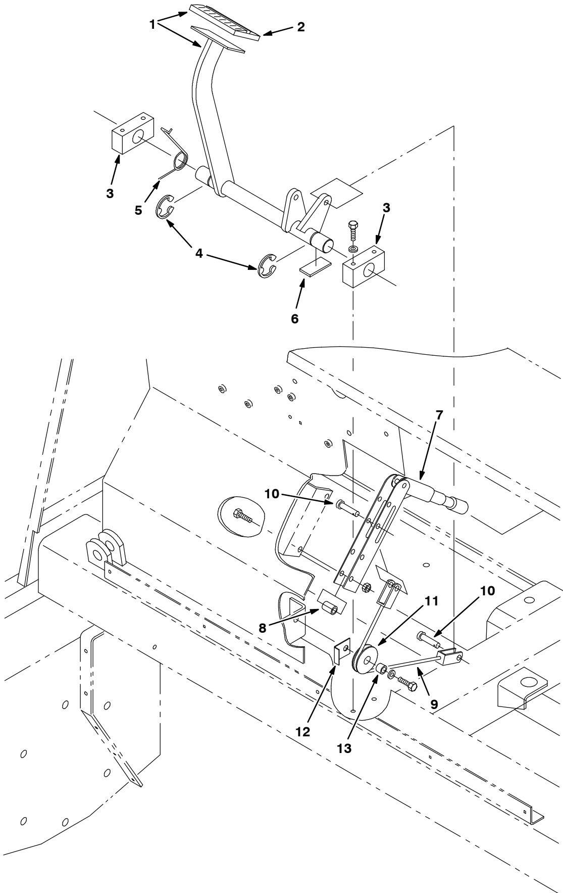
Fig. 35 - Brake Lever and Pedal Group
