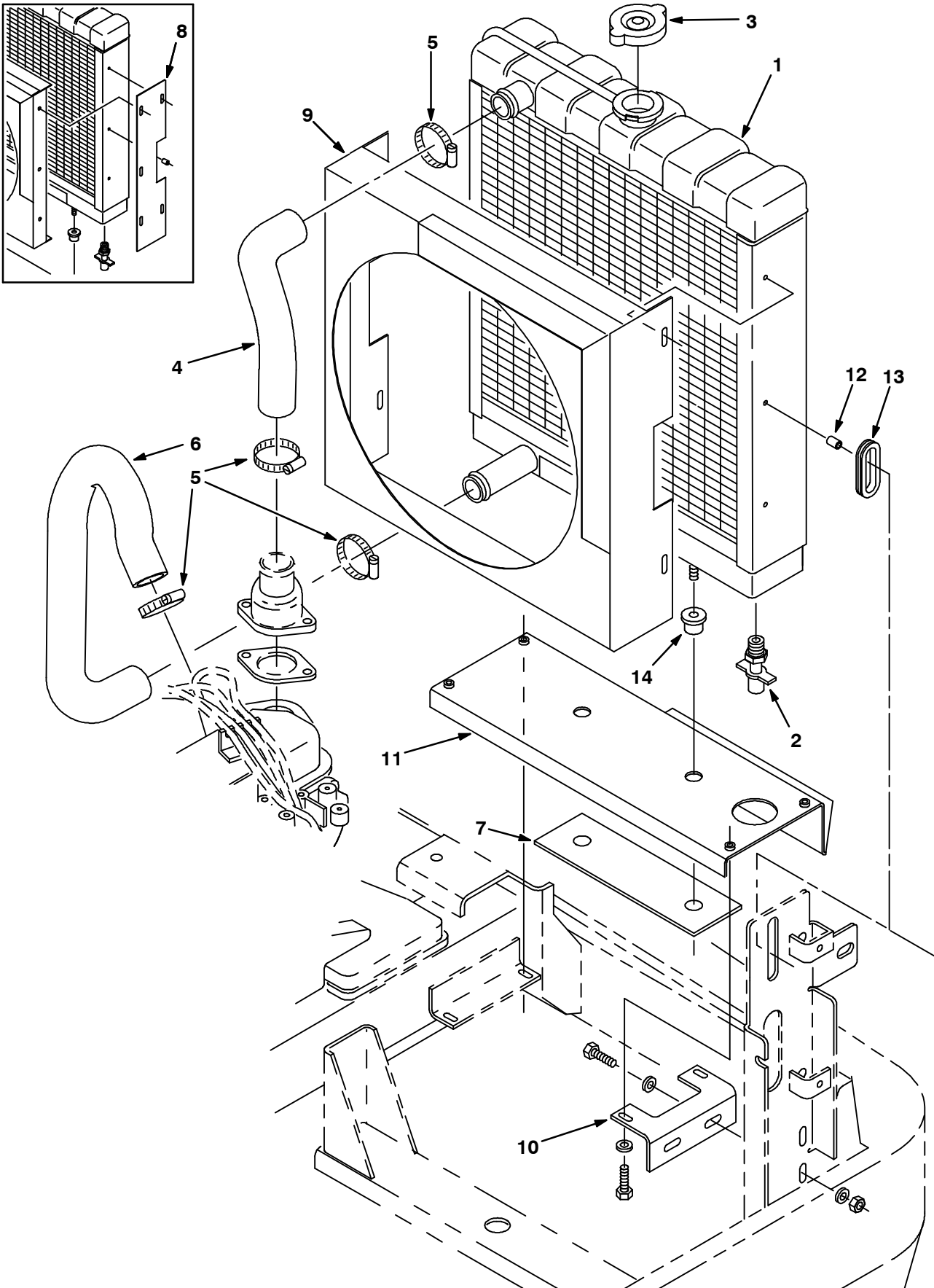
Fig. 29 - Radiator Group
