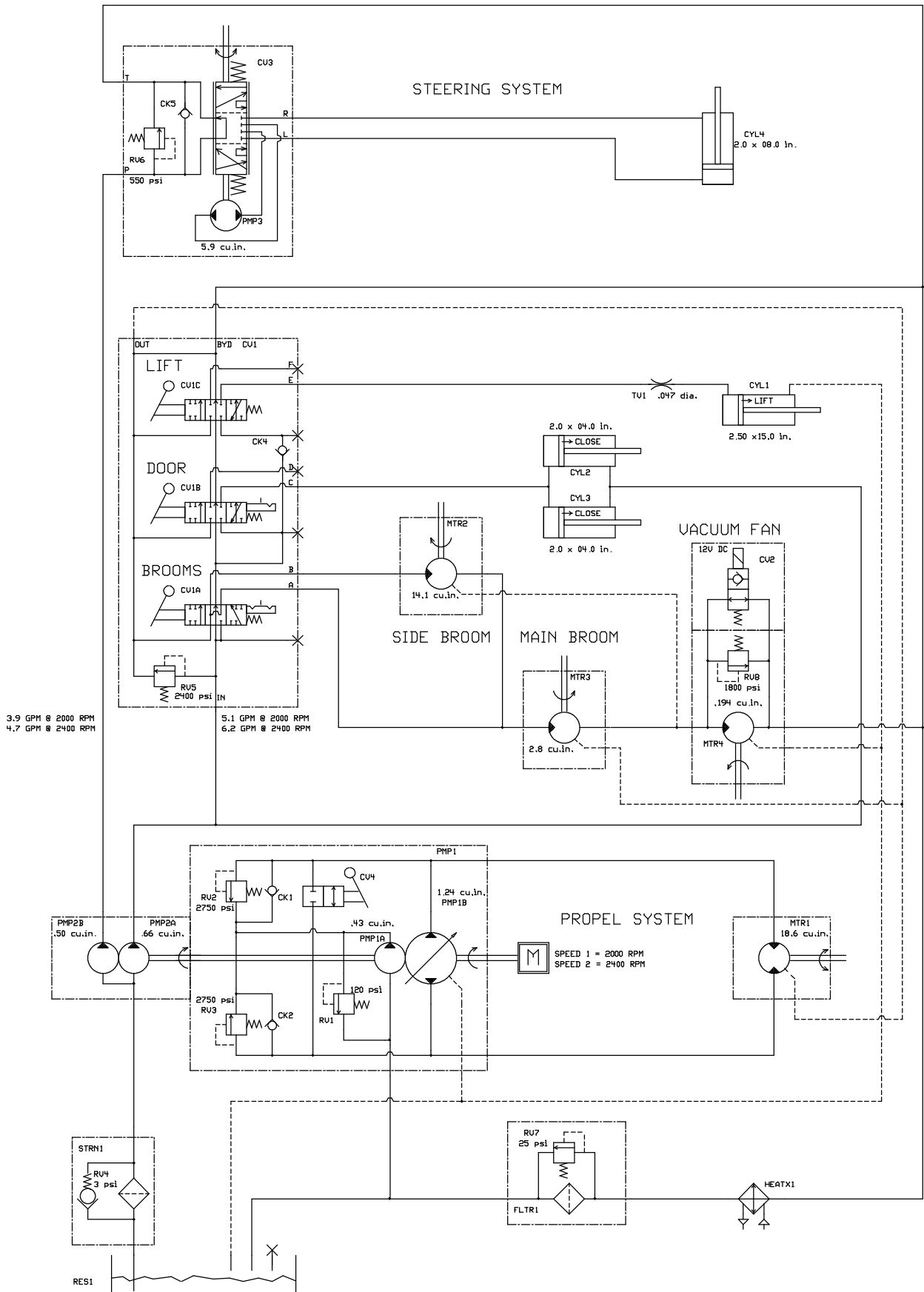
Fig. 50 - Hydraulic Schematic
