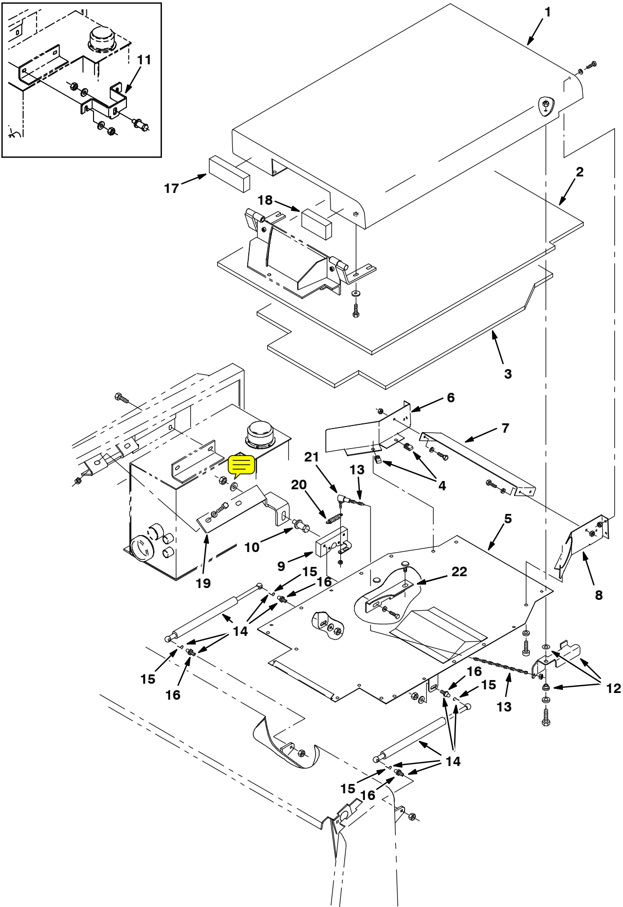
Fig. 9 - Engine Cover Group
